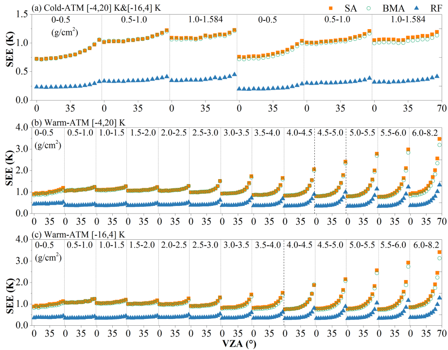
Figure 6. SEE values of the three ensemble methods for NOAA-14 AVHRR under different atmospheric and VZA conditions. (a) Cold-ATM for T_s - NSAT within [-4, 20] K and [-16, 4] K. (b) Warm-ATM for T_s - NSAT within [-4, 20] K. (c) Warm-ATM for T_s - NSAT within [-16, 4] K.
