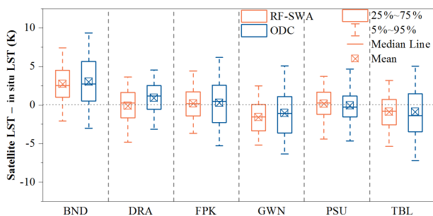
Figure 10. Residuals with respect to in situ LST for ODC and RF-SWA LST for six SURFRAD sites (BND, DRA, FPK, GWN, PSU, and TBL). Details about the sites are provided in Table 4.
