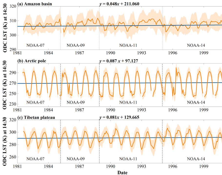
Figure 12. Monthly averaged ODC LST time series normalized to 14:30 ST for 1981–2000 over the Amazon basin (a), the north pole (b), and the Tibetan Plateau (c).
