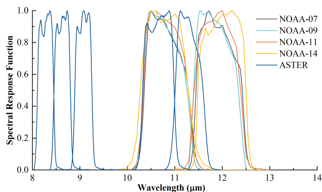
Figure 1. Spectral response functions of NOAA-07, 09, 11, and 14 AVHRR and Terra ASTER.
